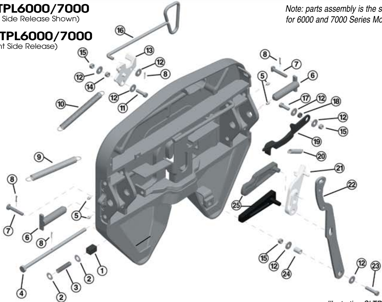
Illustration SLTPL6000
