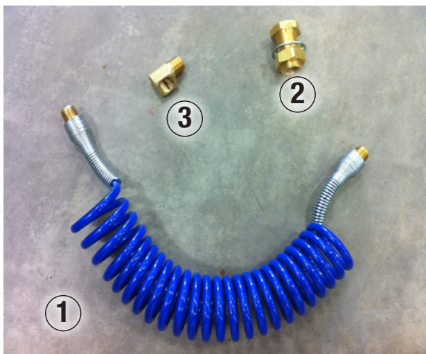
Figure 1: Air line coil kit
