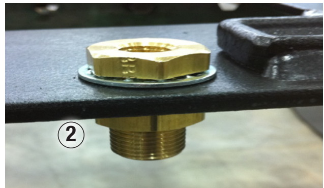
Figure 2: Bulkhead fitting in slot in slide rail
