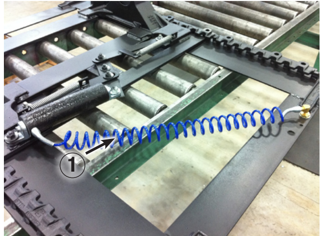
Figure 7: Completed air line coil assembly
