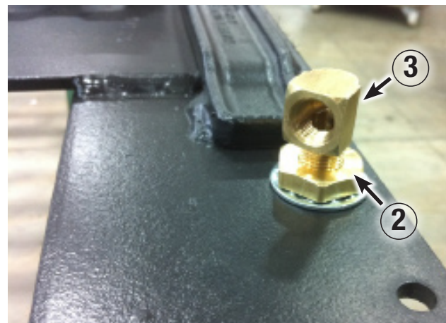
Figure 3: 90° street elbow screwed into bulkhead fitting
